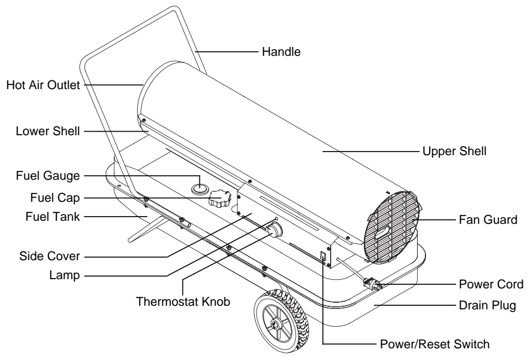
Figure 2. DFA-125T MODEL
