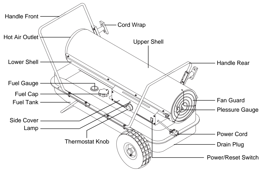
Figure 3. DFA-170C/210C MODELS
