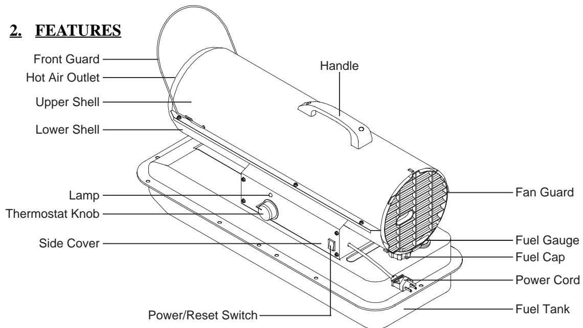
Figure 1. DFA-45T / DFA-70T MODELS
