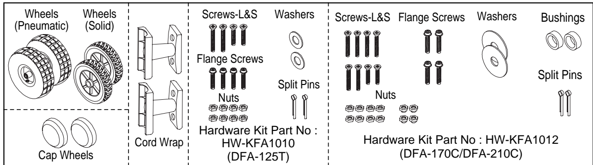
Figure 5. DFA-125T / DFA-170C / DFA-210C MODELS
