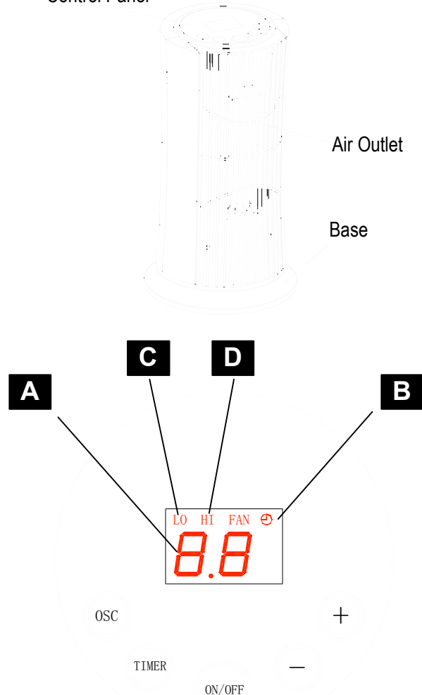
Control Panel
